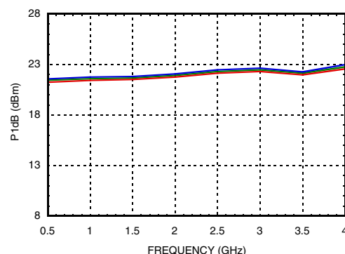
Output P1dB vs. Temperature
